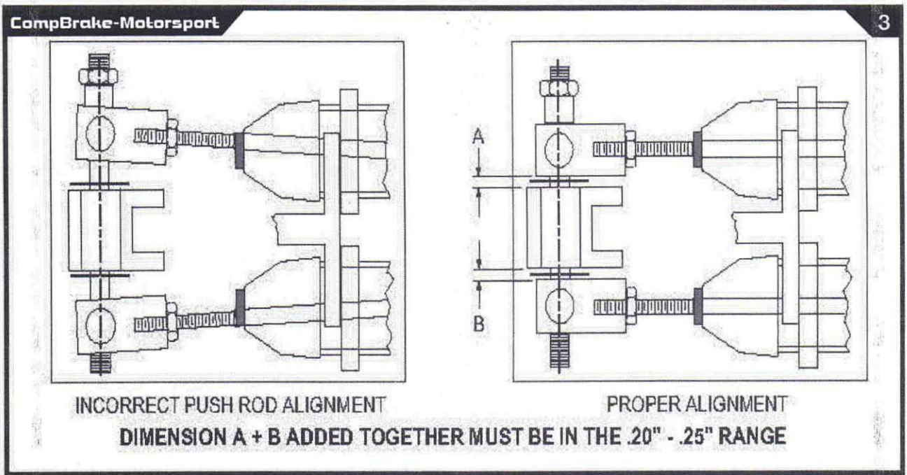
Figure 3 - Example of pushrod alignment.
