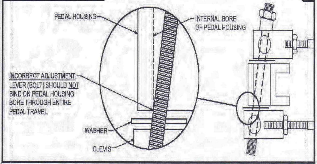
Figure 2 - Balance bar lever interference.
