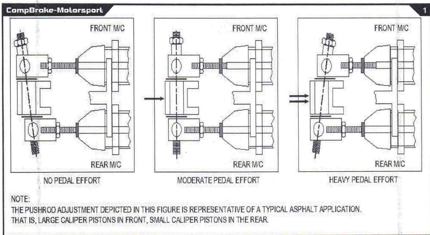
Figure 1 - Balance bar lever adjustment.
